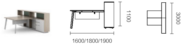
FNR51.16/18/19 1600 × 3000 × 1100 / 1800 × 3000 × 1100 / 1900 × 3000 × 1100
