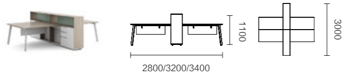
FNR53.28/32/34 2800 × 3000 × 1100 / 3200 × 3000 × 1100 / 3400 × 3000 × 1100
