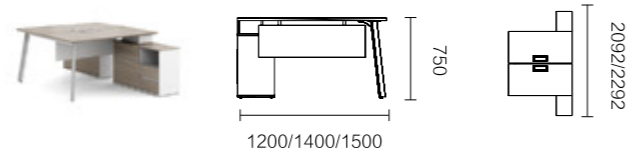
FNR69.12/14/15 1200 × 2092 × 750 / 1400 × 2292 × 750 / 1500 × 2292 × 750
