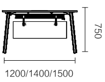
FNR60.12/14/15 1200 × 600 × 750 / 1400 × 700 × 750 / 1500 × 700 × 750 FNR62.12/14/15 1200 × 1212 × 750 / 1400 × 1412 × 750 / 1500 × 1412 × 750
