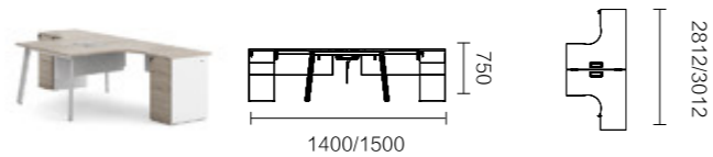
FNR55.14/15 1400 × 2812 × 750 / 1500 × 3012 × 750
