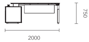
FMQ80L.20 2000 × 1900 × 750
