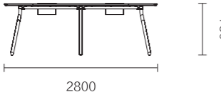
FMQ72.28 2800 × 1200 × 750
