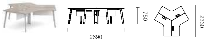
FNR56.26 2690 × 2330 × 750
