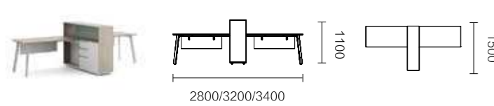
FNR52.28/32/34 2800 × 1500 × 1100 / 3200 × 1500 × 1100 / 3400 × 1500 × 1100
