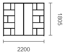
FNQ91.20 2200 × 400 × 1805
