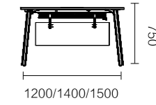
FNR62.12/14/15 1200 × 1212 × 750 / 1400 × 1412 × 750 / 1500 × 1412 × 750
