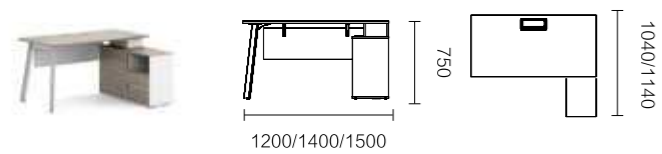
FNR68R.12/14/15 1200 × 1040 × 750 / 1400 × 1140 × 750 / 1500 × 1140 × 750
