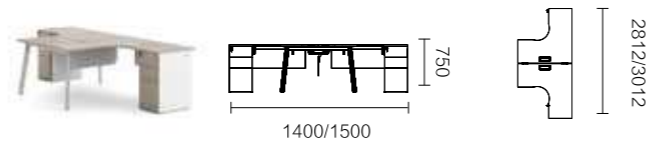
FNR55.14/15 1400 × 2812 × 750 / 1500 × 3012 × 750
