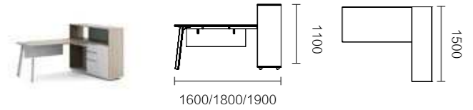
FNR50R.16/18/19 1600 × 1500 × 1100 / 1800 × 1500 × 1100 / 1900 × 1500 × 1100
