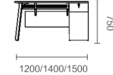
FNR67.12/14/15 1200 × 1212 × 750 / 1400 × 1412 × 750 / 1500 × 1412 × 750
