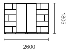
FNQ91.26 2600 × 400 × 1805
