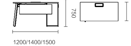
FNR66R.12/14/15 1200 × 600 × 750 / 1400 × 700 × 750 / 1500 × 700 × 750
