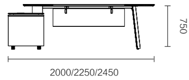
FNR81R.22/24 2250 × 1850 × 750 / 2450 × 1850 × 750
