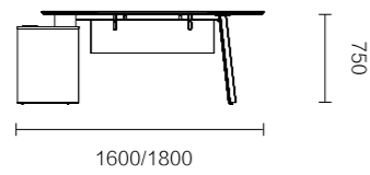
FNR80R.16/18/20 1600 × 1300 × 750 / 1800 × 1300 × 750 / 2000 × 1650 × 750
