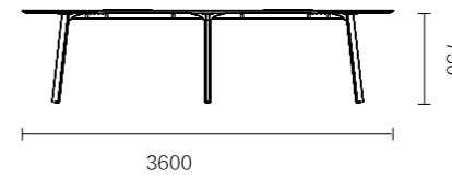
FNR72.30 3600 × 1200 × 750
