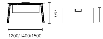
FNR60.12/14/15 1200 × 600 × 750 / 1400 × 700 × 750 / 1500 × 700 × 750
