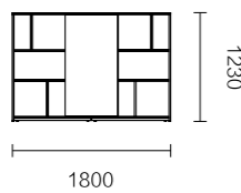
FNQ90.18 1800 × 400 × 1230
