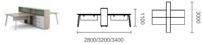
FNR53.28/32/34 2800 × 3000 × 1100 / 3200 × 3000 × 1100 / 3400 × 3000 × 1100
