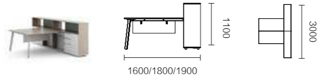
FNR51.16/18/19 1600 × 3000 × 1100 / 1800 × 3000 × 1100 / 1900 × 3000 × 1100
