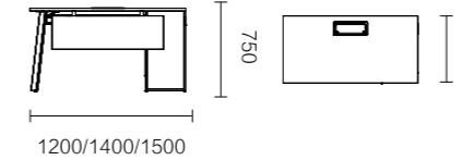
FNR64.12/14/15 1200 × 600 × 750 / 1400 × 700 × 750 / 1500 × 700 × 750
