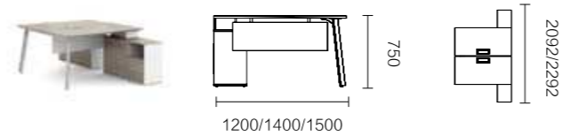
FNR69.12/14/15 1200 × 2092 × 750 / 1400 × 2292 × 750 / 1500 × 2292 × 750
