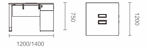
FNQ67.12BJ/FNQ67.14BJ 1200 × 1200 × 750 / 1400 × 1200 × 750
