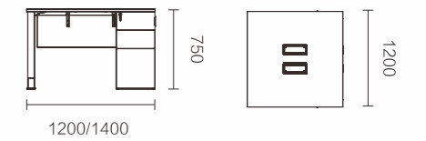
FNQ63.12BJ/FNQ63.14BJ 1200 × 1200 × 750 / 1400 × 1200 × 750
