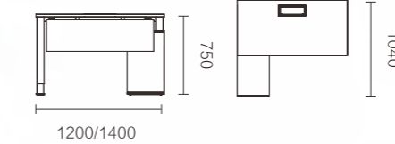
FNQ64L.12BJ/FNQ64L.14BJ 1200 × 1040 × 750 / 1400 × 1040 × 750
