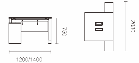
FNQ65L.12BJ/FNQ65L.14BJ 1200 × 2080 × 750 / 1400 × 2080 × 750
