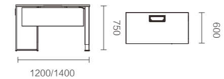
FNQ66L.12BJ/FNQ66L.14BJ 1200 × 600 × 750 / 1400 × 600 × 750
