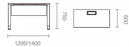
FNQ60.12BJ/FNQ60.14BJ 1200 × 600 × 750 / 1400 × 600 × 750
