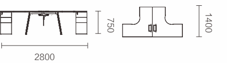
FNQ53.28BJ 2800 × 1400 × 750
