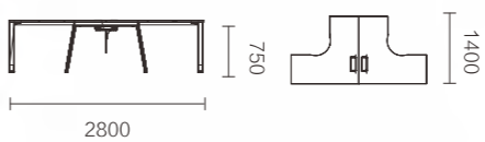
FNQ51.28BJ 2800 × 1400 × 750
