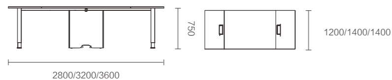
FNQ72.28BJ/32BJ/36BJ 2800 × 1200 × 750 / 3200 × 1400 × 750 / 3600 × 1400 × 750
