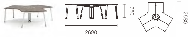
FNQ58.28BJ 2680 × 2680 × 750
