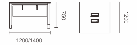
FNQ62.12BJ/FNQ62.14BJ 1200 × 1200 × 750 / 1400 × 1200 × 750
