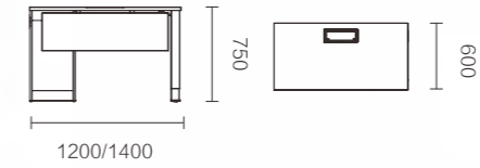
FNQ61.12BJ/FNQ61.14BJ 1200 × 600 × 750 / 1400 × 600 × 750
