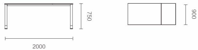
FNQ70.20BJ 2000 × 900 × 750
